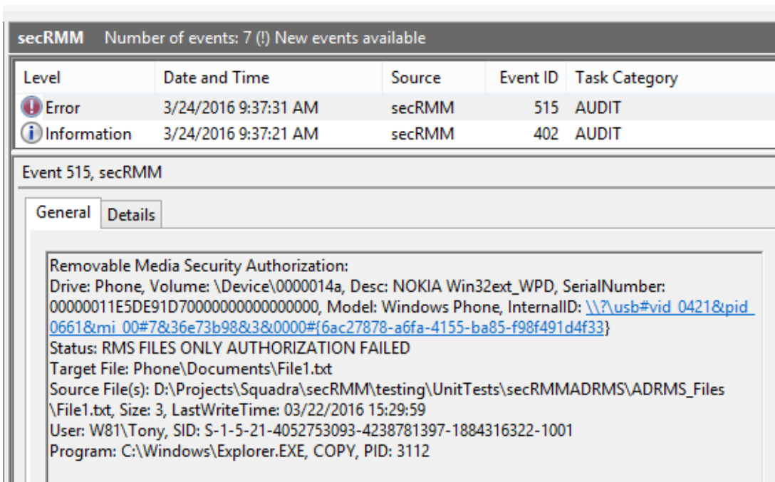
Figure 16 - secRMM Allow RMS Files Only
