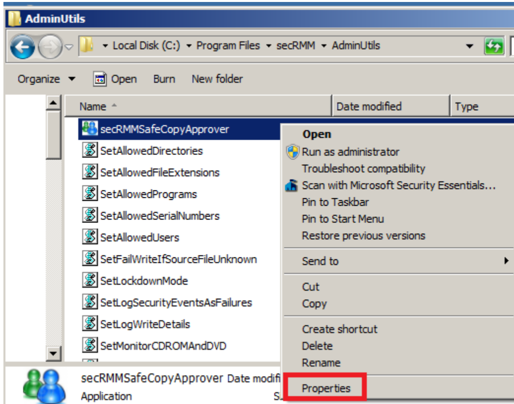
Figure 43 - secRMMSafeCopyApprover Properties
