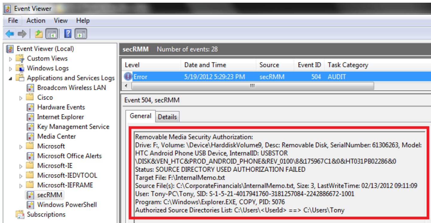
Figure 13 - secRMM Source Directory Authorization failed event
